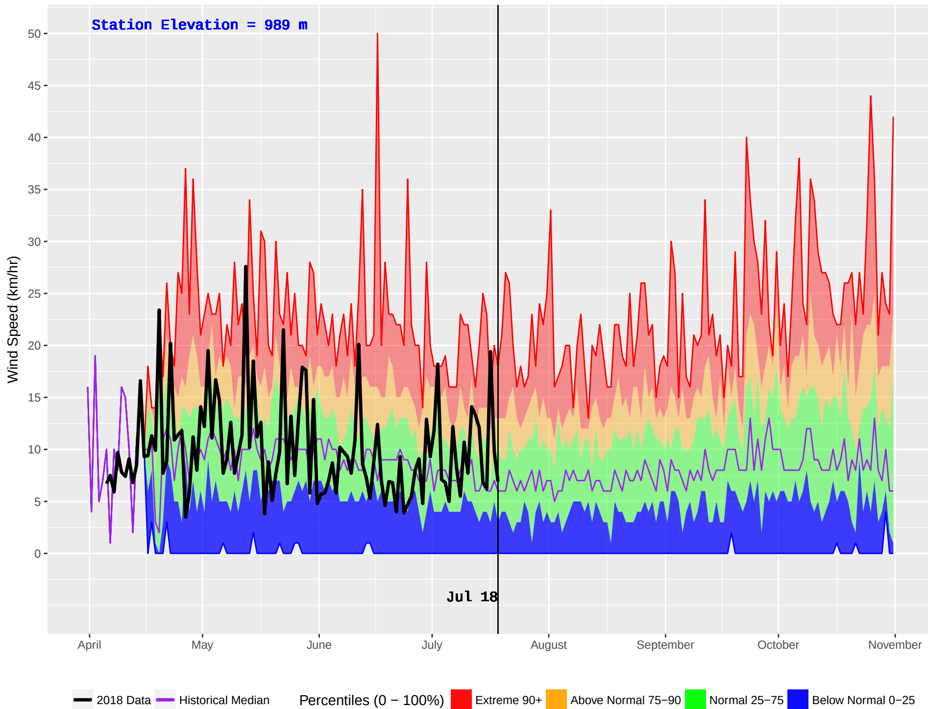
PINK MOUNTAIN (129) : Historical (1983–2016) and Current (2018) Daily Wind Speed
