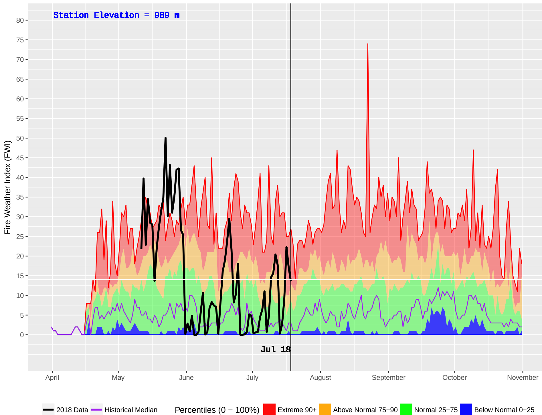
PINK MOUNTAIN (129) : Historical (1983–2016) and Current (2018) Daily Fire Weather Index (FWI)
