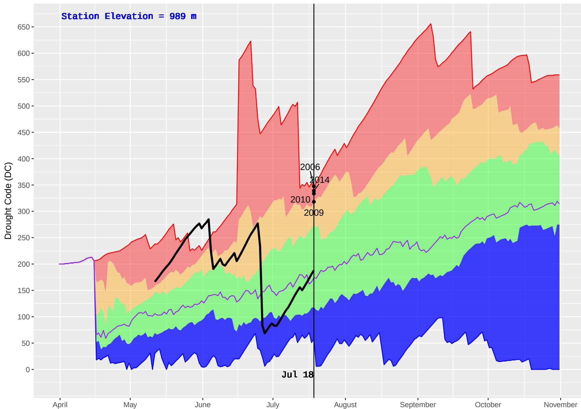
PINK MOUNTAIN (129) : Historical (1983–2016) and Current (2018) Daily Drought Code (DC)
