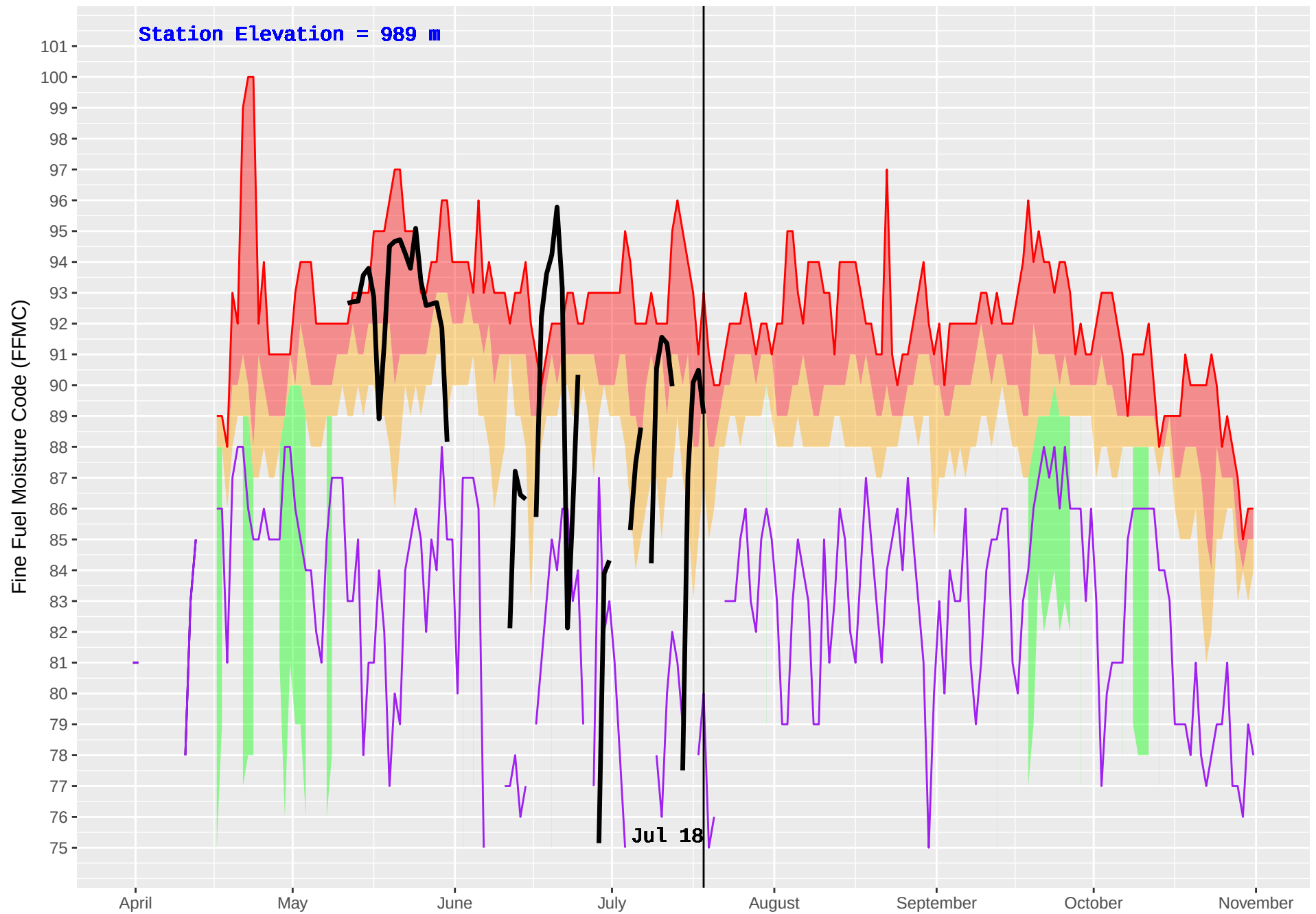
PINK MOUNTAIN (129) : Historical (1983–2016) and Current (2018) Daily Fine Fuel Moisture Code (FFMC)
